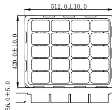
Blister tray
