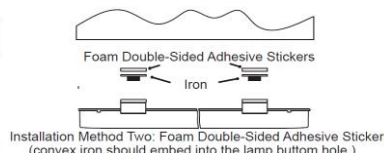
Installation Method Two: Foam Double-Sided Adhesive Stickers (convex iron should embed into the lamp bottom hole)
