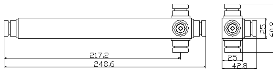
Figure 1 JX-PS-575-6000-XCNI Power Divider
