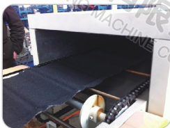
4. Auto face glue spraying section
