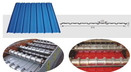
齿形浪板打拱机 Tooth shape corrugated sheet bending machine
