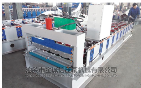
JCX21-215-860彩钢瓦成型机 Color Steel Roll Forming Machine
