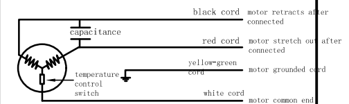
motor wiring diagram
