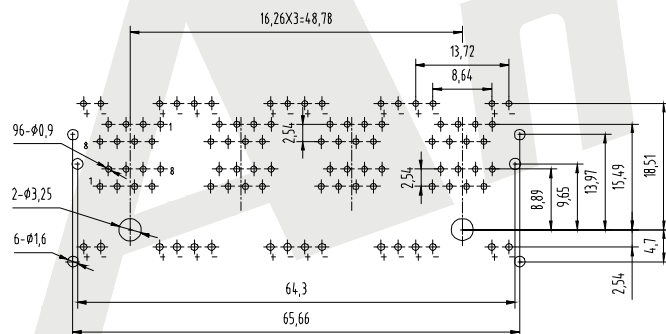
PC Board Layout Component Side Shown
