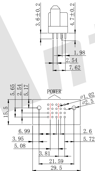
P. C. Body Hole Layout
