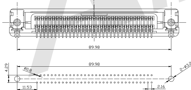
PCB Layout
