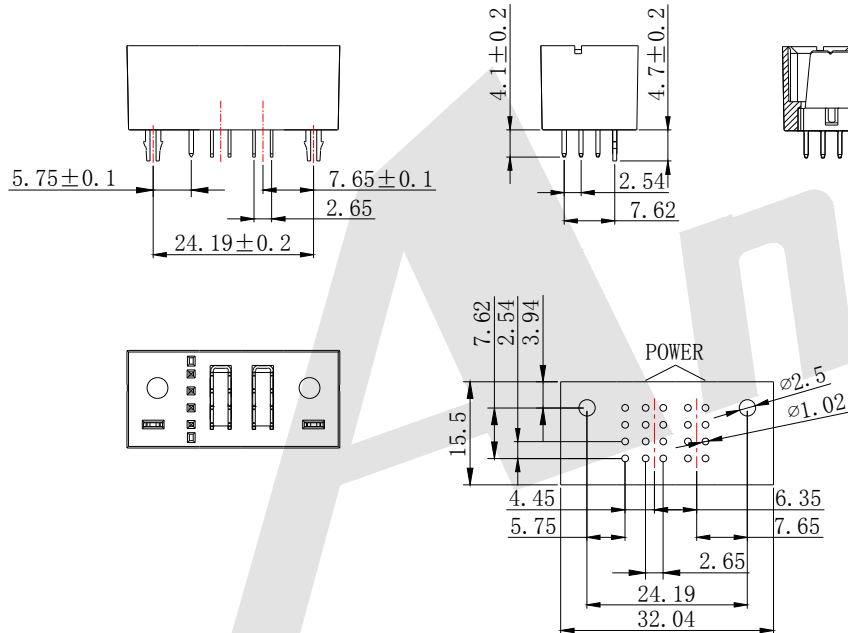
P. C. Body Hole Layout
