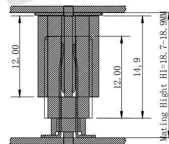
Mating Draw(Ref)
