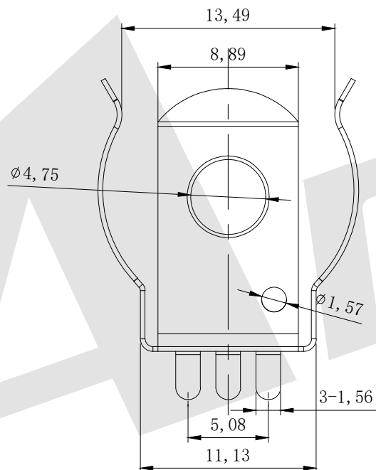
MOUNTING LAYOUT
