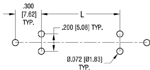
MOUNTING LAYOUT
