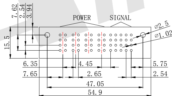
P. C. Body Hole Layout
