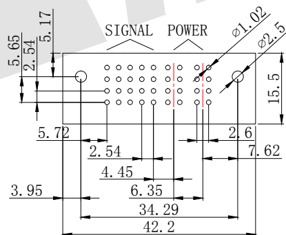
P.C. Body Hole Layout
