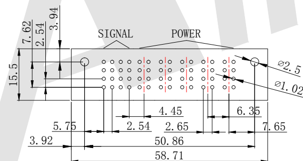
P. C. Body Hole Layout
