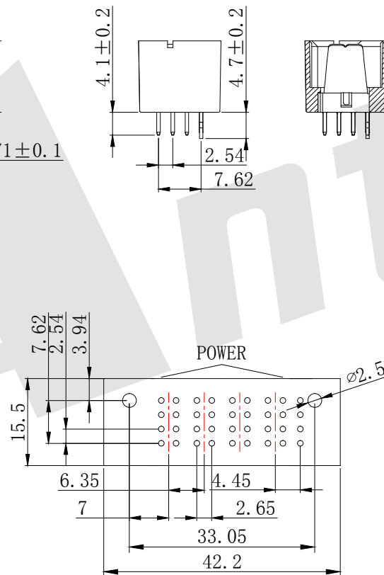
P. C. Body Hole Layout
