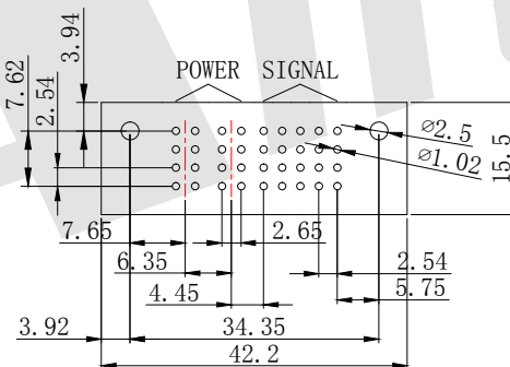
P. C. Body Hole Layout
