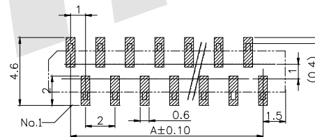
TYPE B PCB LAYOUT
