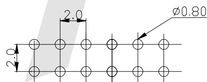
PCB Hole Layout
