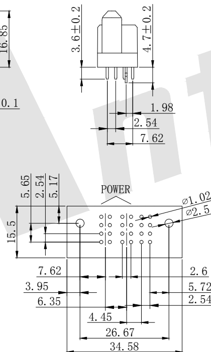
P. C. Body Hole Layout
