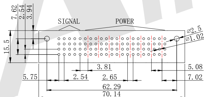
P.C. Body Hole Layout
