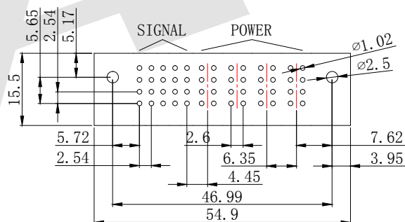
P. C. Body Hole Layout
