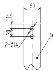
LV terminal
