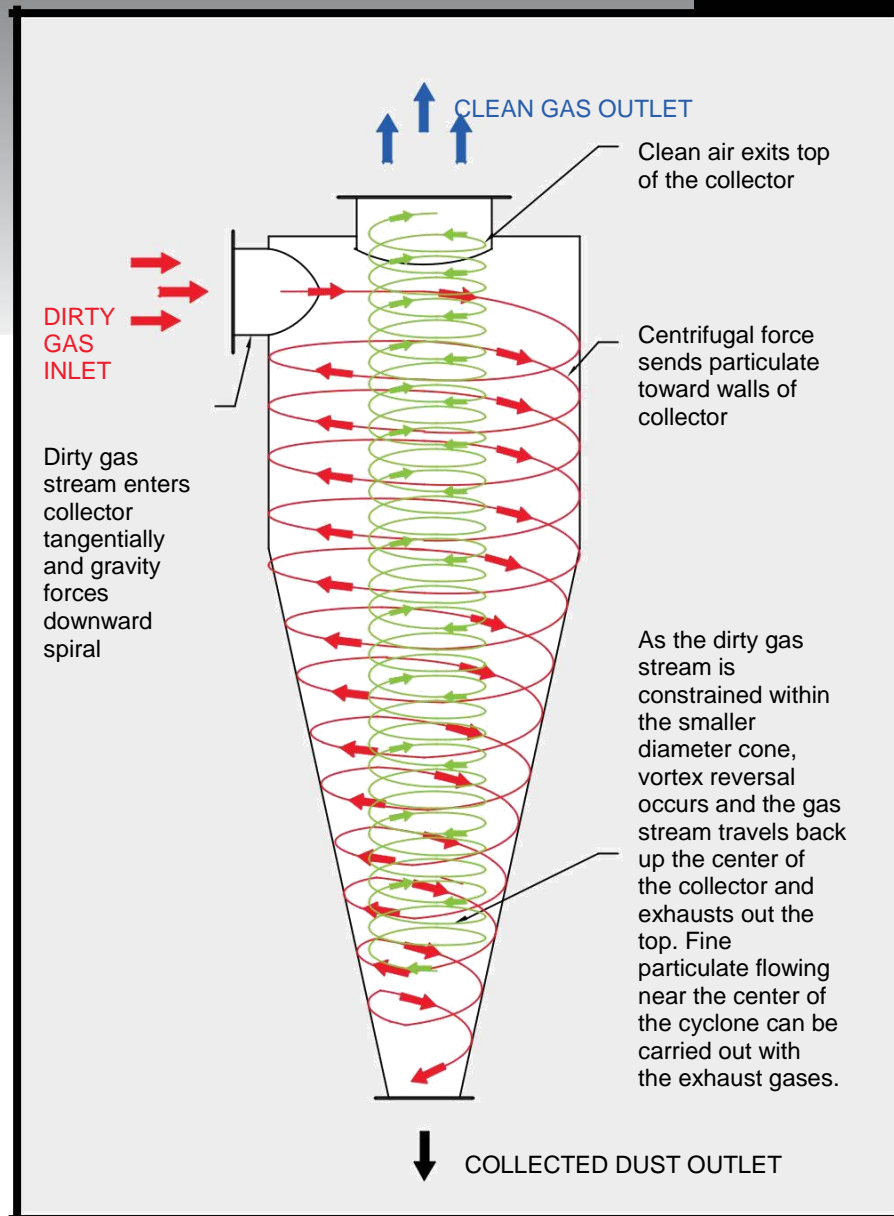
Standard Cyclone Dust Collector
