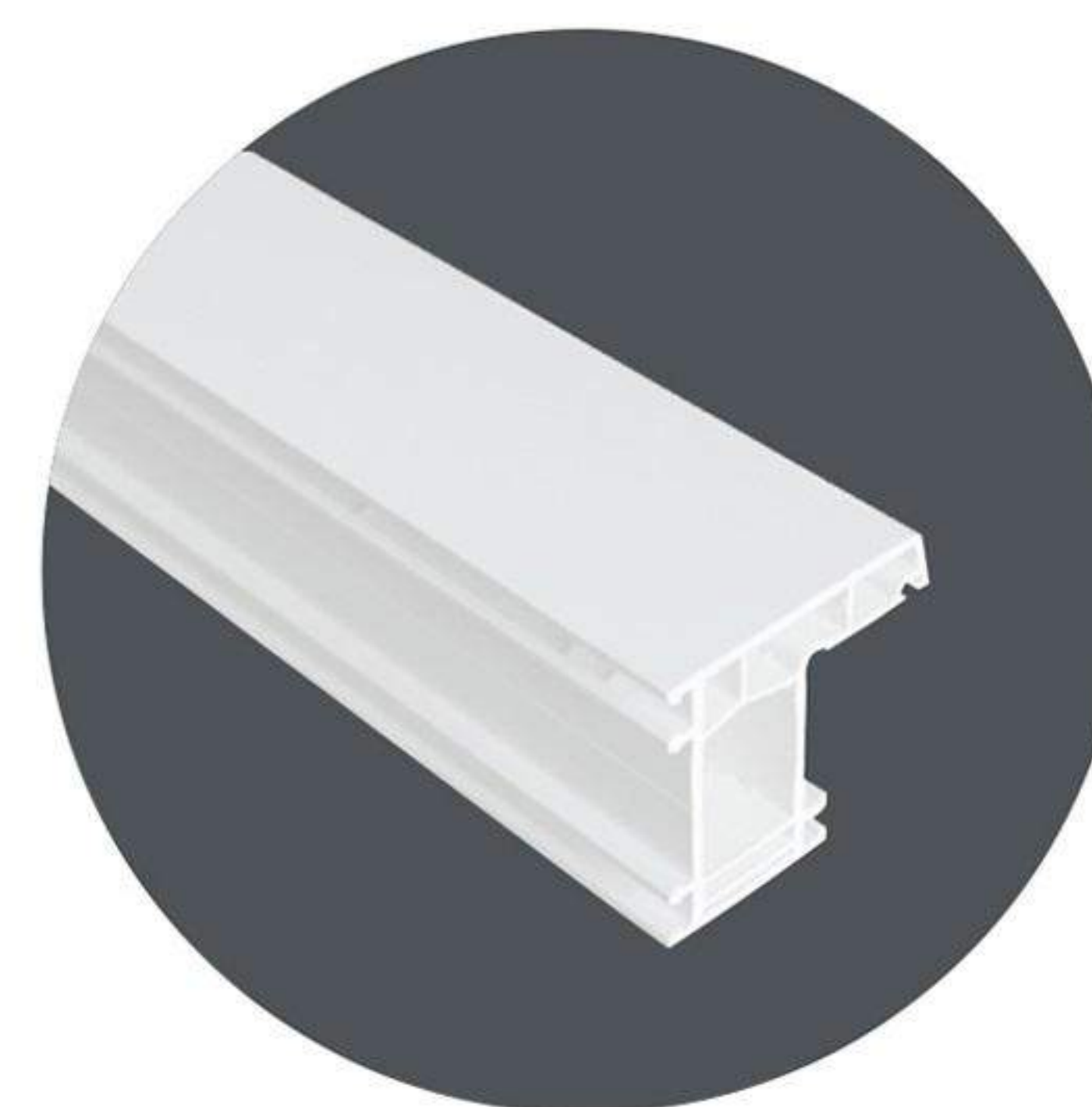
60 三密封平开框 60 Three sealed flat open frame
