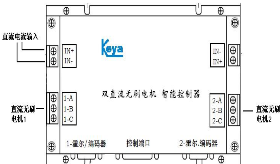
Description of connection terminals
