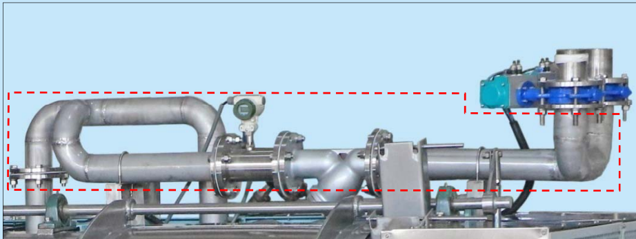
O-I-70-03 入水流量計系統-Ø3" Water inlet flow meter system - Ø3"
