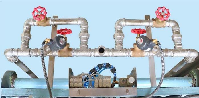
蒸汽(直接/間接加溫)氣動閥總成 Steam (Direct/Indirect Heating) Pneumatic Valve Assy
