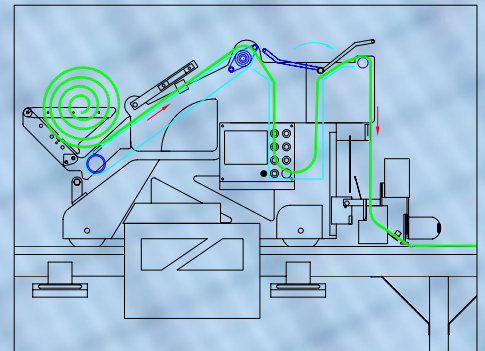
送布原理圖 Fabric Feeding Illustration
