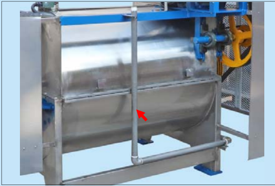
蒸汽直接加溫裝置(NS-2700-70~100) Direct steam heating device (NS-2700-70~100)
