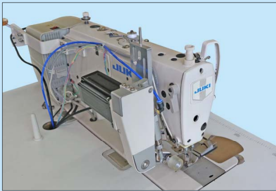
A801安裝后外觀 Appearance of A801 after installation
