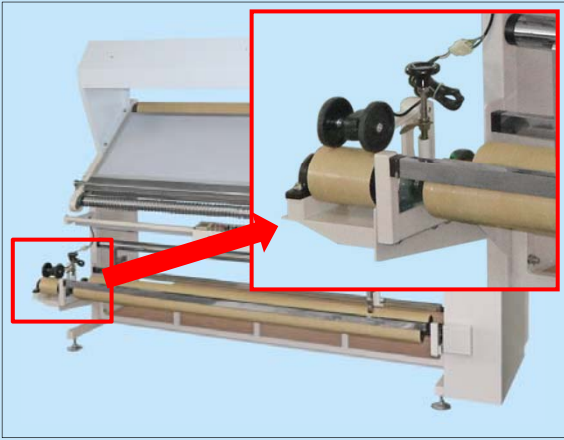
布碼計數表可根據客戶需要安裝於左側 Fabric length meter can be mounted on the left side at customer's request
