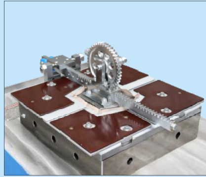
袋蓋模四邊同時摺壓 Pocket flap mould creases all sides
