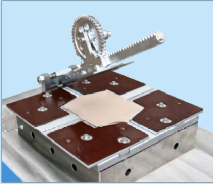
將袋布放在發熱板上 Place material on heating platform
