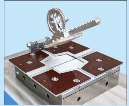
袋蓋摺壓完成 Pocket flap creasing finished
