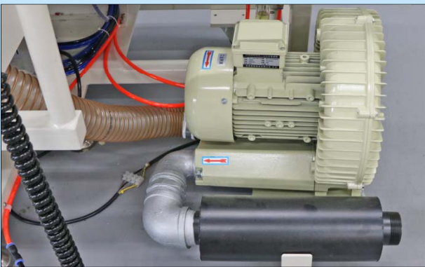
真空泵抽濕定位 Vacuum pump for vacuuming and fabric positioning
