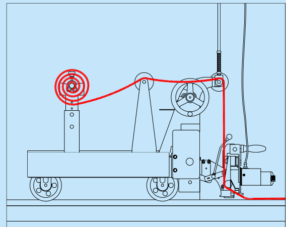
穿布圖 Loading cloth diagram
