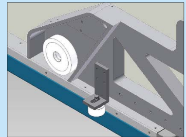
無路軌裁床与拉布機配合原理圖 Work Principle of Cloth Spreader & Cutting Table without Track
