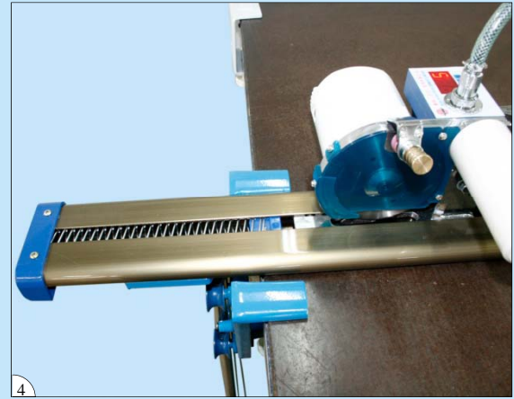
4 回彈裝置 Rebounding device
