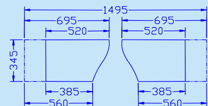
下模尺寸簡圖 Dimension Diagram of the Lower mould
