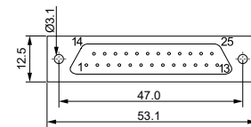
插孔 Female 25 Pin
