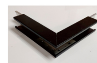
Inner corner connector 明装薄导轨外转角驳接件 FW-CXPJ004 170x170x27.4mm black
