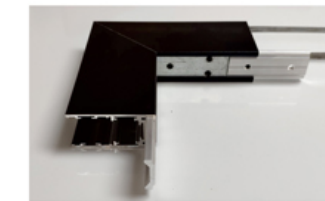
Outer corner connector 明装高边导轨外转角驳接件 FW-CXPJ008 170x170x54.5mm black
