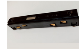
Straight current collector 对接接电器 FW-CXJDQ002 18.6x16.1x119.5mm black
