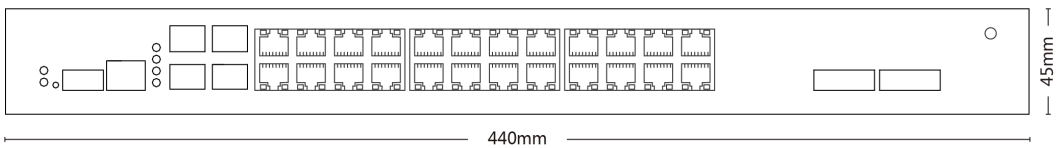
Front view
