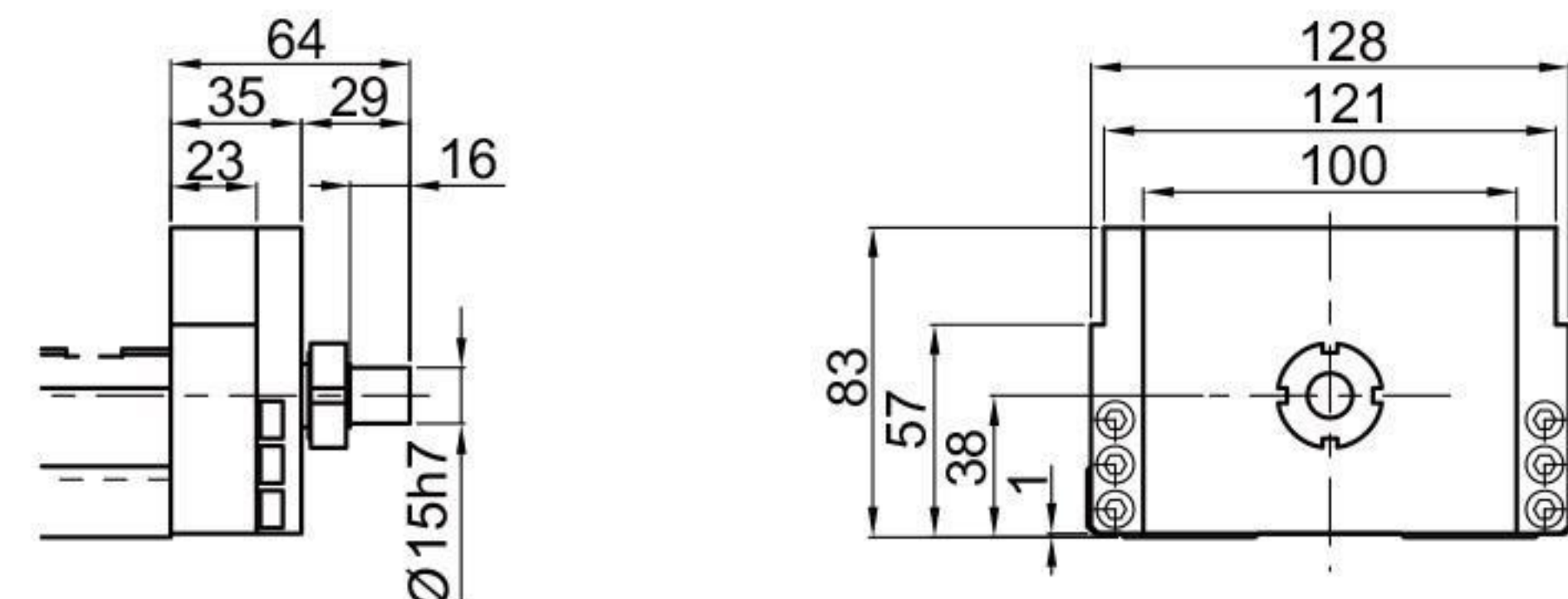
Motor Housing H0
