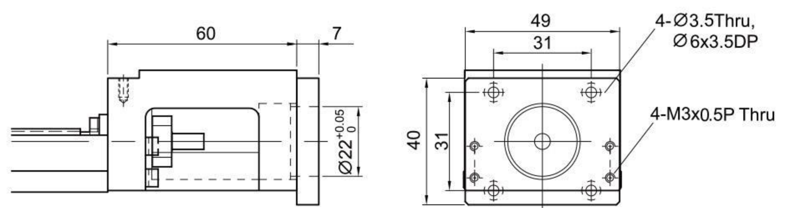
Motor Adaptor Flange F3
