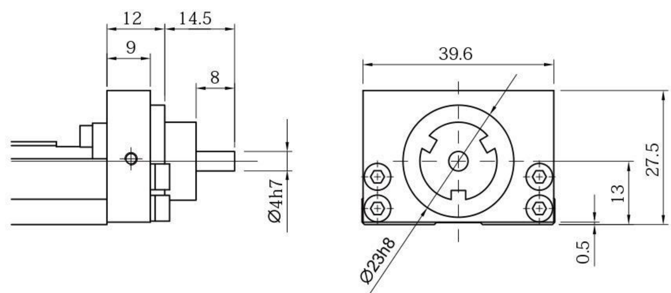
Motor Housing H0
