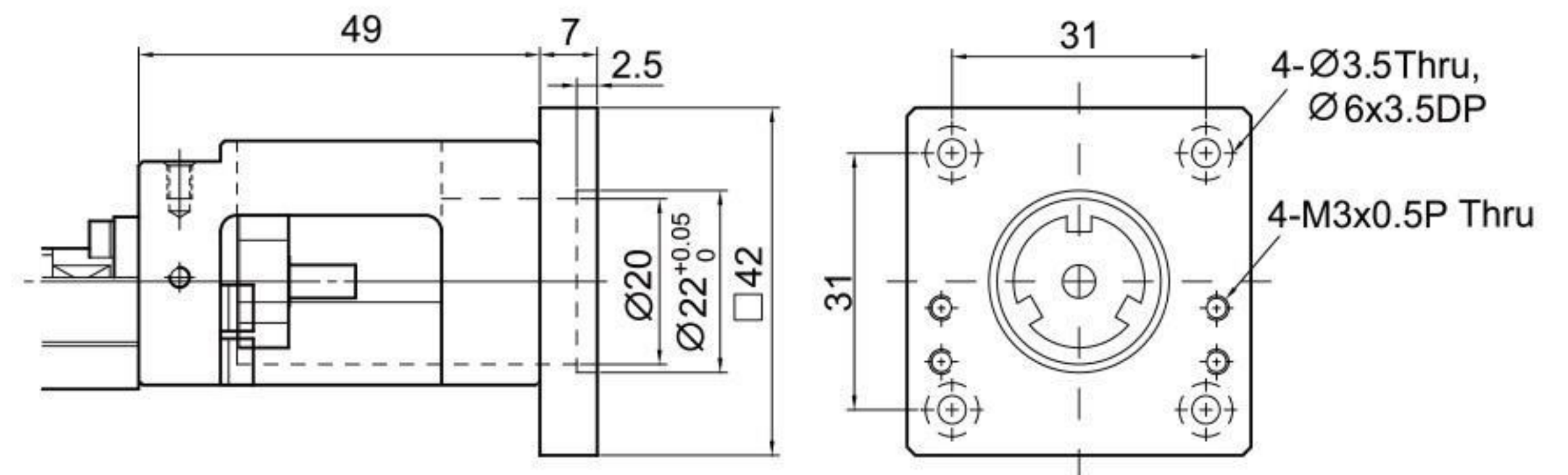
Motor Housing H0
