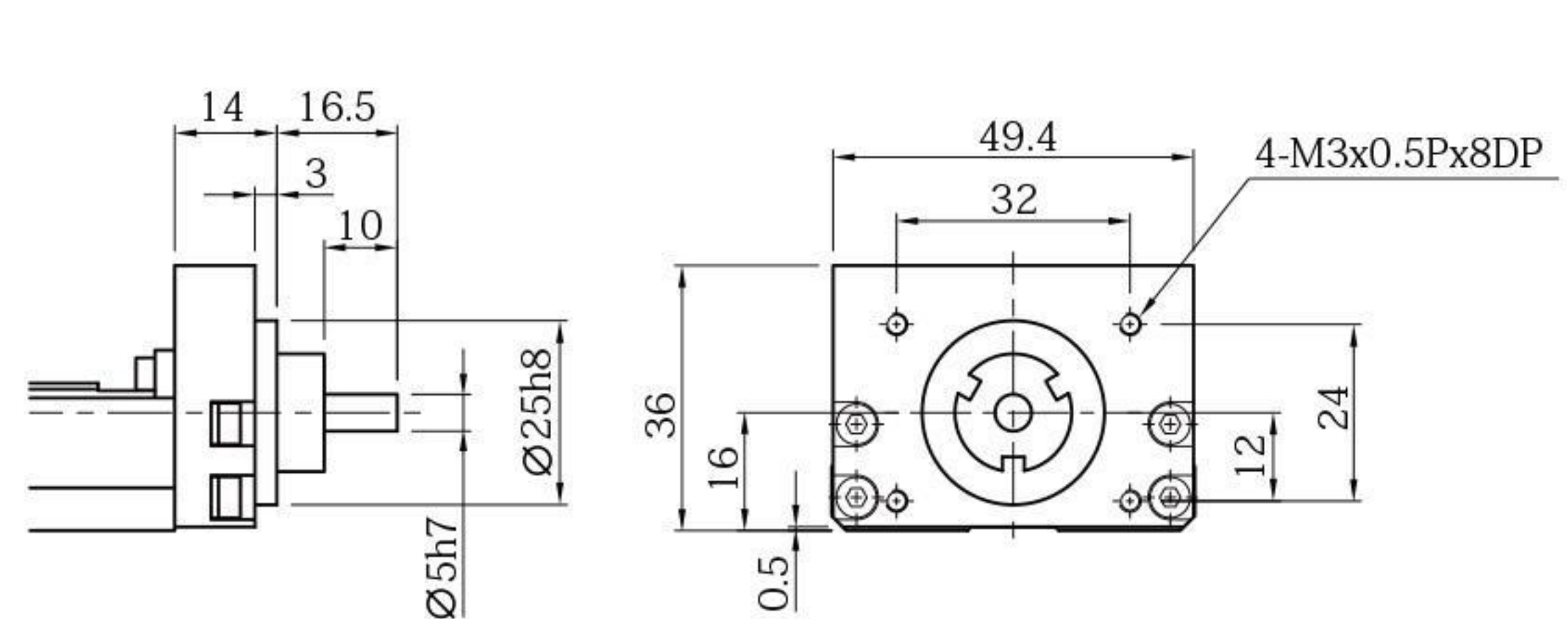
Motor Housing H0
