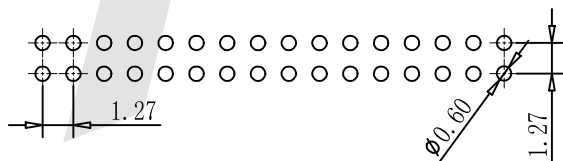
Recommended P.C.B Layout(Top Side) (PCB BOARD TOLERANCE±0.05)
