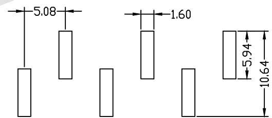
TYPE B PCB LAYOUT
