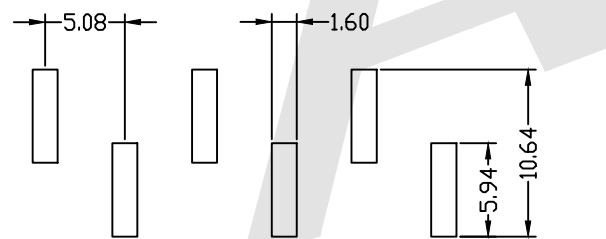
TYPE A PCB LAYOUT
