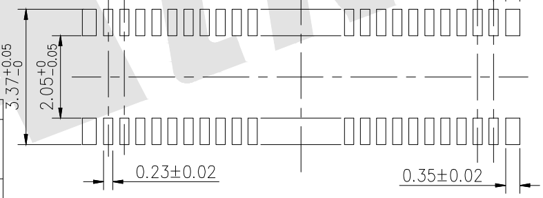
Recommended PC board pattern (TOP VIEW)
