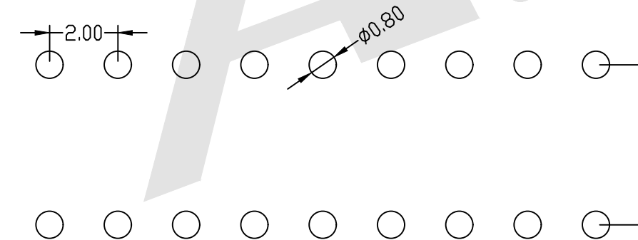
PCB LAYOUT
