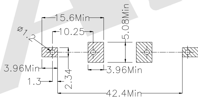
Scale:2:1 PCB Layout Diagram Top View
