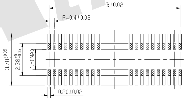
Recommended PC board pattern (TOP VIEW)
