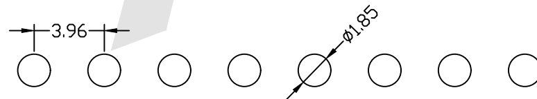
PCB LAYOUT
