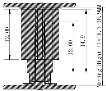
Mating Draw(Ref)
