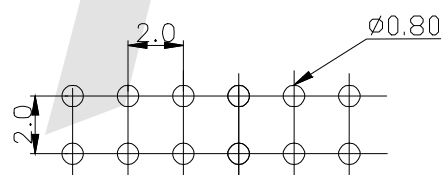
PCB Hole Layout
