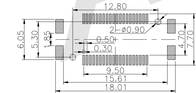
Recommended P.C.Board Layout (Tolerance:±0.05)
